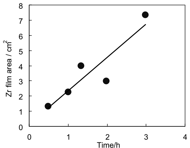
Fig. 6. Relationship between the Zr film area and the electrolysis time.
