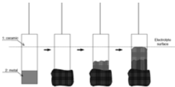
Fig. 4. Formation process of Zr film on ceramic.
