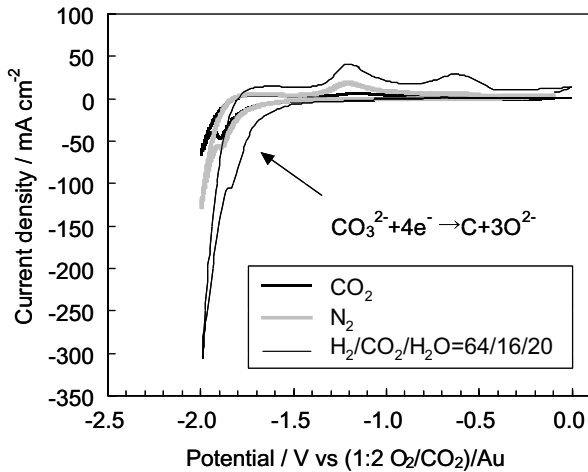
Fig. 8. Cyclic voltammograms for Au electrode in \text{Li}_2\text{CO}_3\text{-Na}_2\text{CO}_3 eutectic melt at 650\text{ }^\circ\text{C} , scan rate 0.1\text{ V s}^{-1} . Gas compositions are \text{H}_2/\text{CO}_2/\text{H}_2\text{O} = 64/16/20 , \text{CO}_2 and \text{N}_2 .
